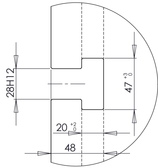
DETAIL B SCALE 1 : 2
